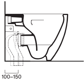
cod. 90 5456 0000 Adjustable pipe elbow fitting.
