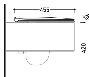
art. AS118G vista laterale / lateral view
