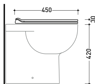
art. QK117G - QK117RG vista laterale / lateral view
